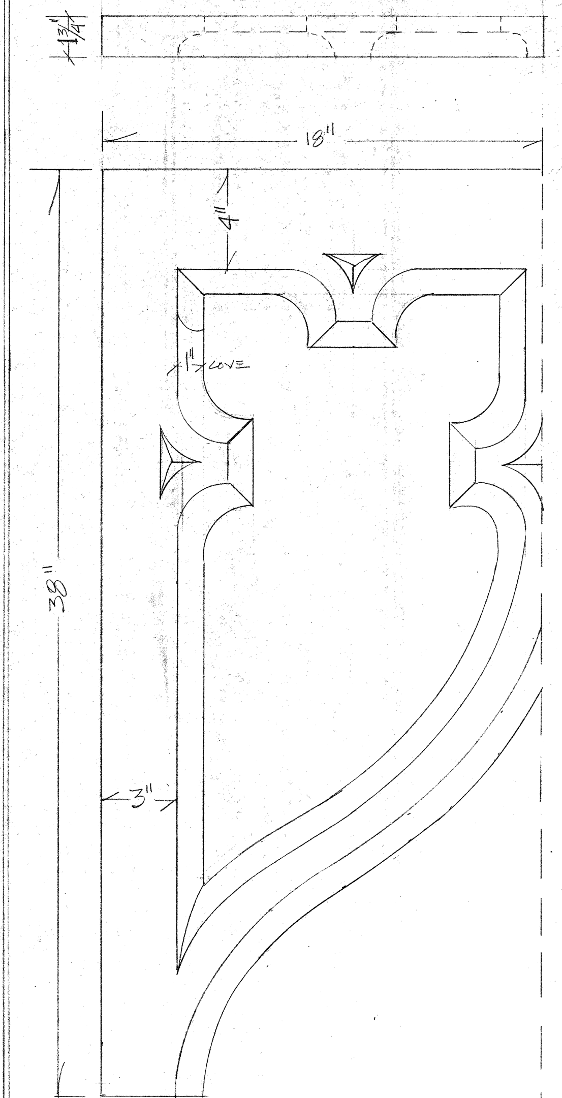
TRACERY DETAIL SCALE: 1/4" = 1" TEMPLATE PROVIDED TO WOODWORKERS BY DESIGNER
